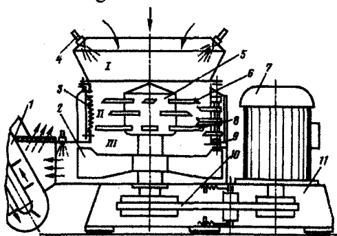
2.2.14-rasm. ISK-3 ozuqa maydalagich-aralashtirgichi:
