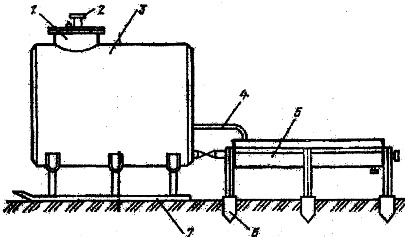
3.2.17-rasm. AGK-12 avtosug'orgich:
