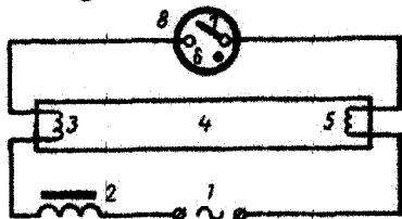
4.3.3-rasm. Lyuminsent lampaning ulanish sxemasi:
