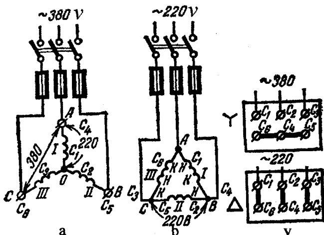
4.2.1 - rasm. Asinxron dvigatelning chulg'amli va uning ulanish sxemalari
