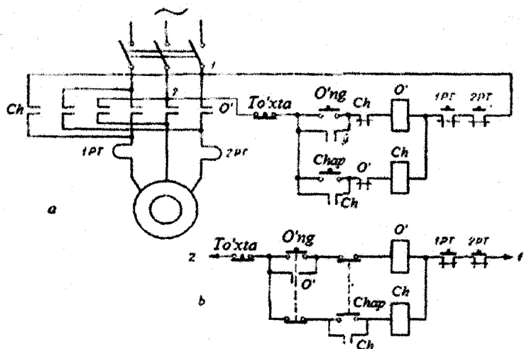
4.2.7 - rasm. Reversiv magnitli ishga tushirgich sxemasi: a) elektr blokirovkali, b) mexanik blokirovkali
