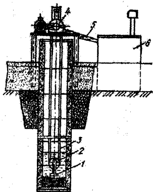
3.2.10-rasm. VLM-100 lentali suv ko'targich:
