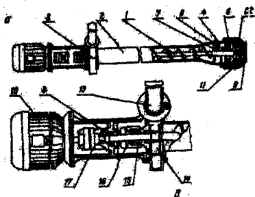
3.5.7-rasm. NSH-50 rusumli shnekli nasos qurilmasining o'rnatilishi va ishlashi:
