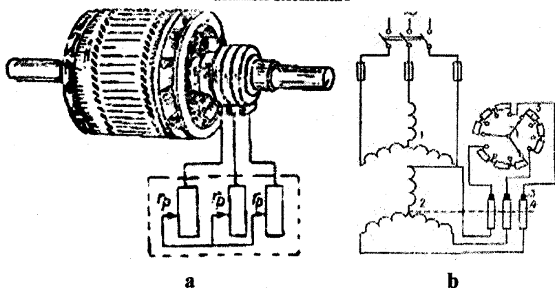
4.2.2 - rasm. Faza rotorli asinxroi dvigatelining ulanish sxemasi
