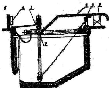
3.5.7-rasm. NSH-50 rusumli shnekli nasos qurilmasining o'rnatilishi va ishlashi:
