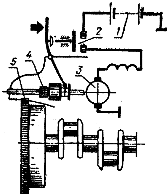
1.2.7 - rasm. Elektr startyor bilan yurgizib yuborish sxemasi: 1-akkumulyatorlar batareyasi; 2-ulagich; 3-elektr startyor; 4-startyor shesternyasi; 5-dvigatel maxovigining tishli g'ildiragi.
