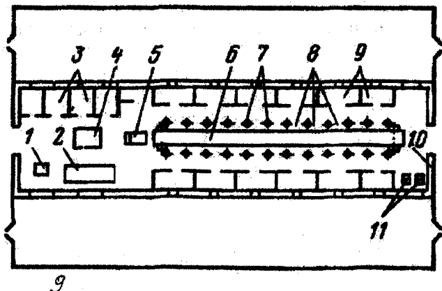
3.8.9-rasm. KTO-24 turg'un jun qirqish punkti:
