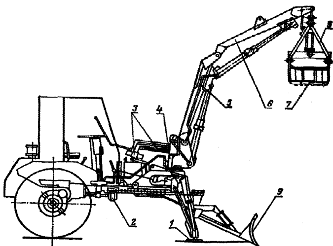
1.4.3 - rasm. PG - 0,2 markali universal greyferli yuklagich: 1-domkratlar; 2-reduktor; 3-gidrotizim; 4-kolonna (ustun) korpusi; 5-strela; 6-ustqo'yma; 7-greyfer; 8-greyfer osmasi; 9-buldozer.
