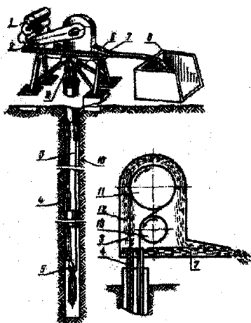
3.2.11-rasm. VSHP-50 rusumli arqonli suv ko'targich:
